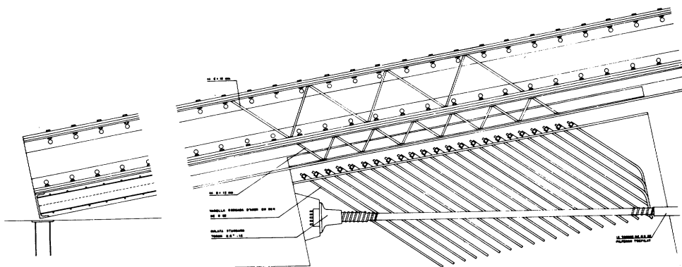
7. Detail of arched segments
