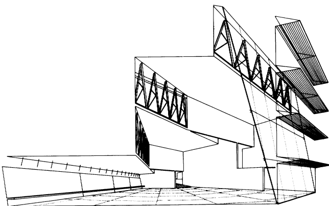
6. Section-perspective
