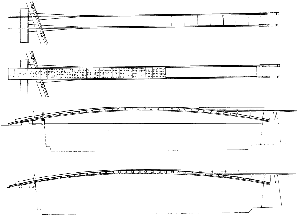
4. Plans and elevations of arched segments
