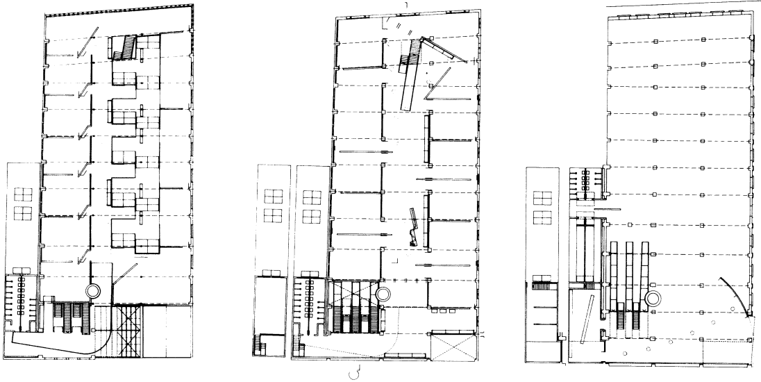
7. Plans
