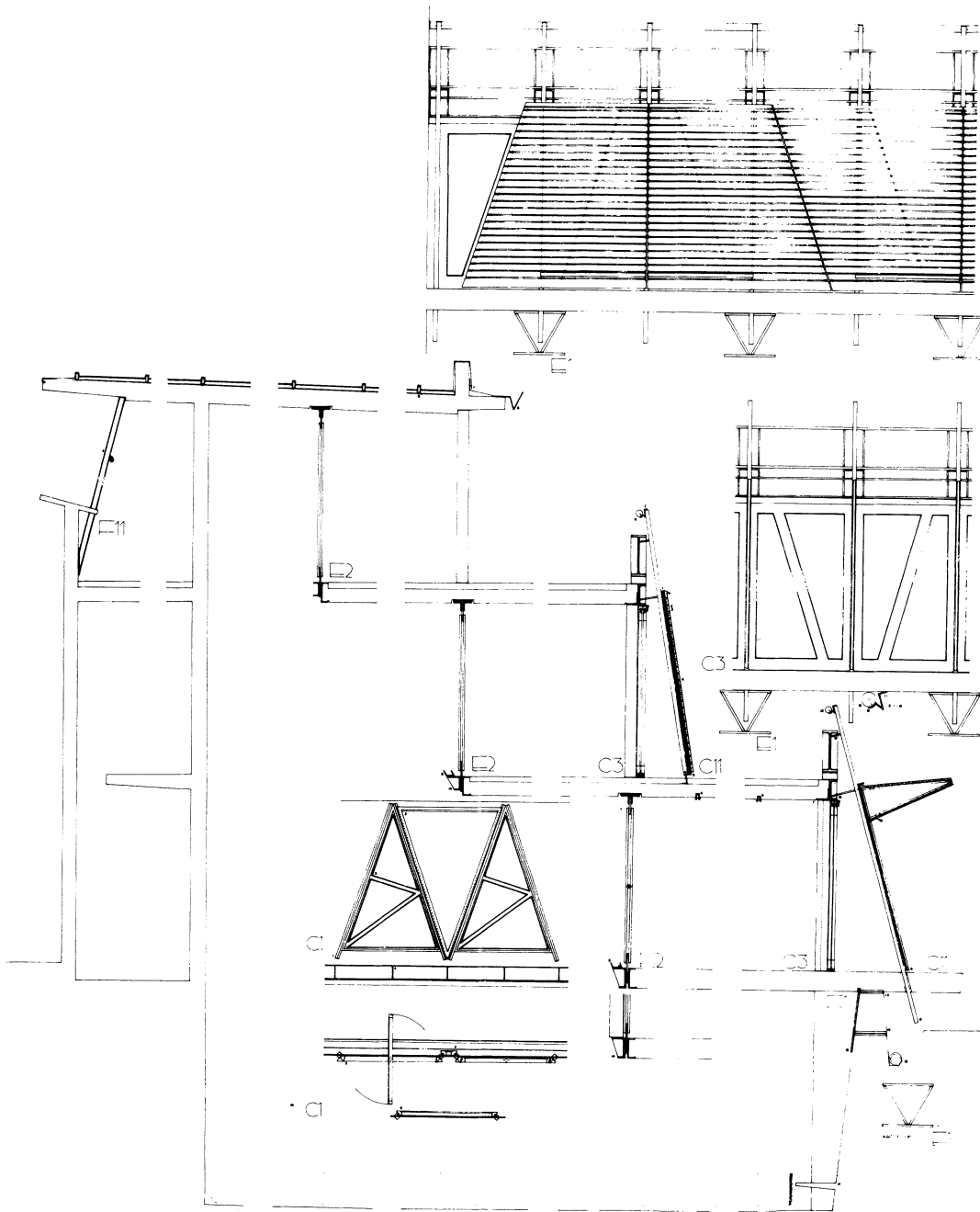
7. Detail of sunscreens
