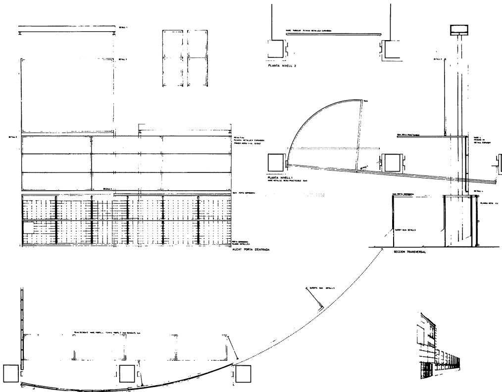
5. Details of sliding door
