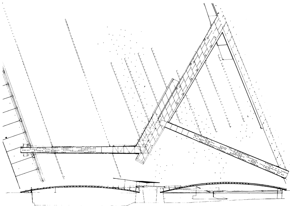
6. Plan with elevation
