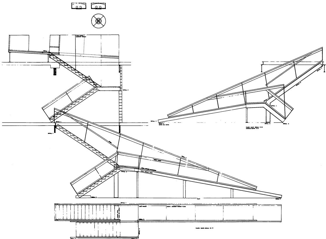
17. Details of the ramp-stairs
